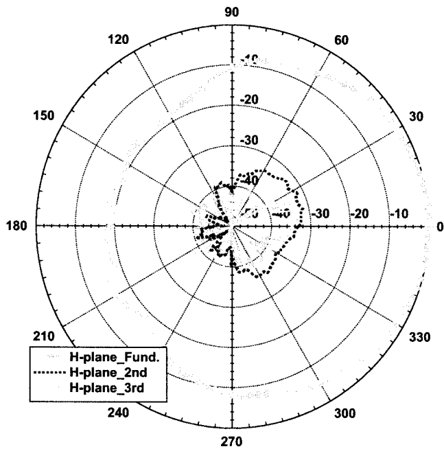
Fig. 9. Measured H -plane radiation patterns at the fundamental of 7.25-GHz, second, and third harmonic frequencies for the AlGaIn/GaN HFET power amplifier integrated with the microstrip circular sector antenna.
