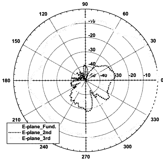
Fig. 10. Measured E -plane radiation patterns at the fundamental of 7.25-GHz, second, and third harmonic frequencies for the AlGaIn/GaN HFET power amplifier integrated with the microstrip circular sector antenna.
