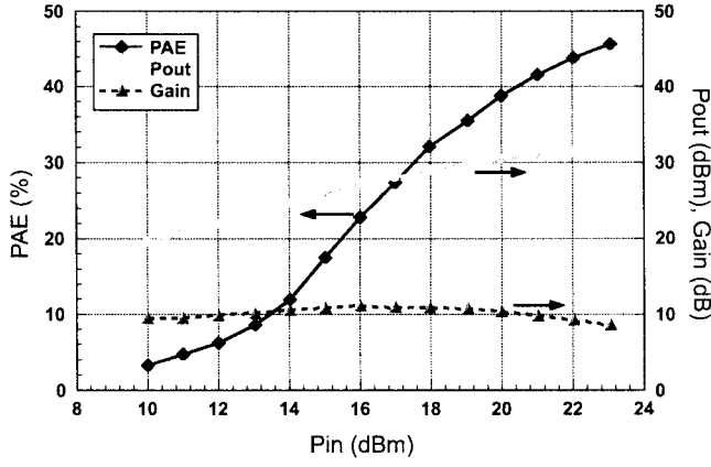
Fig. 3. Measured load-pull large-signal performance with Z_{OPT} load impedance for a 1-mm-wide AlGaN/GaN HFET.
